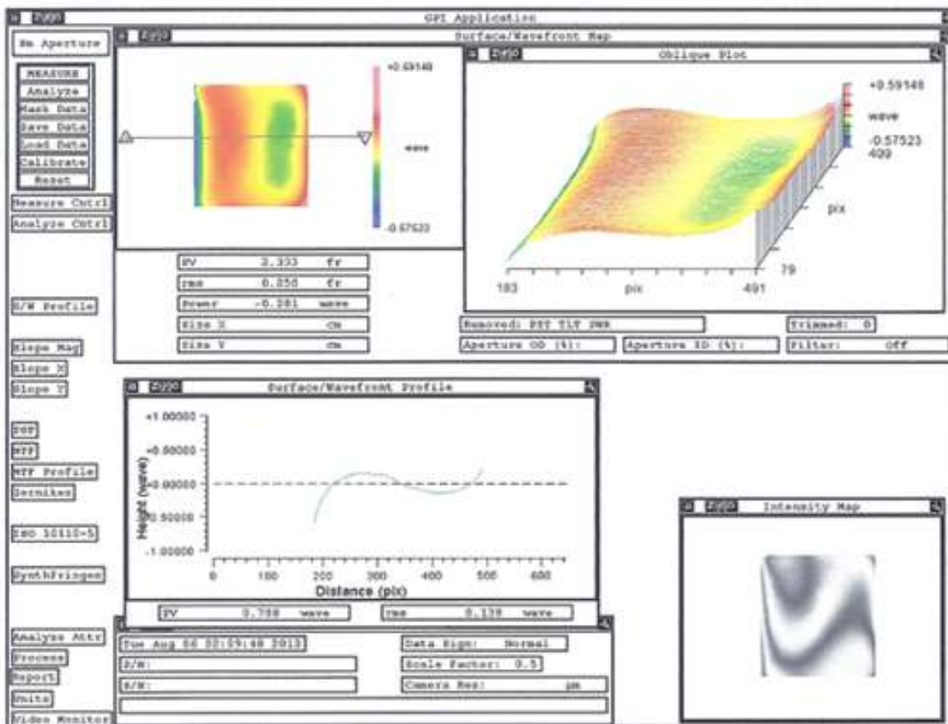
Interferograms made by Zygo GPI XP/D interferometer (632.8 nm HeNe laser light source) showing the Interference Pattern and computerized measured results
